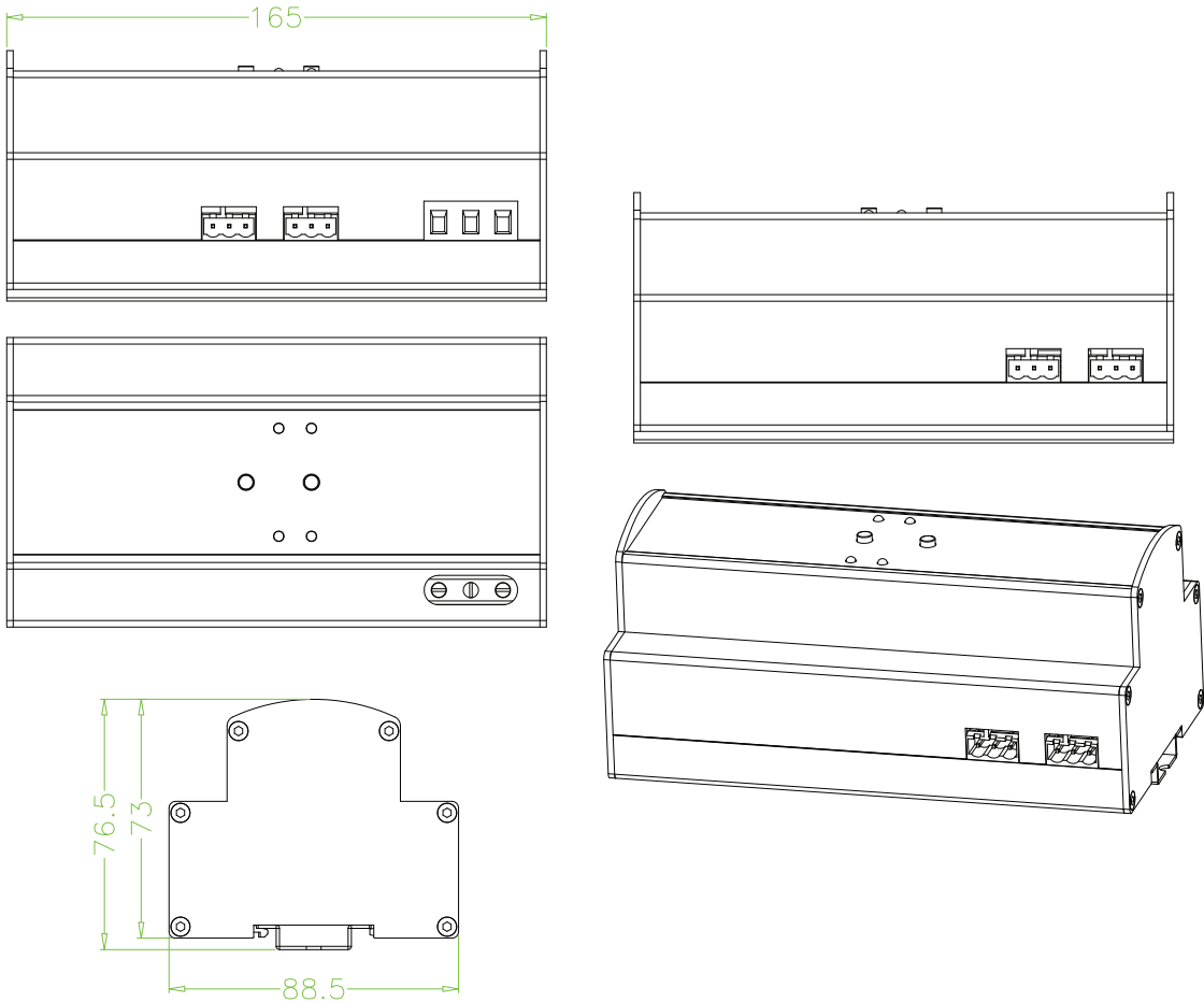
DSX4 DIMENSIONS
