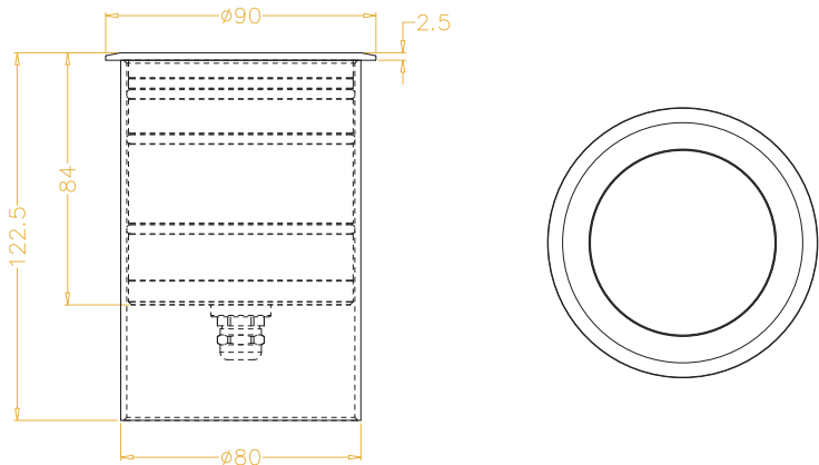
AXS1 - 6 FIXTURE DIMENSIONS
