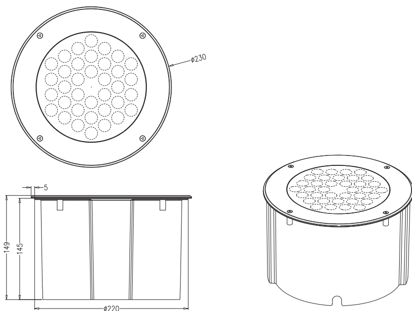
AXS 36 FIXTURE DIMENSIONS – IN-GROUND VERSION
