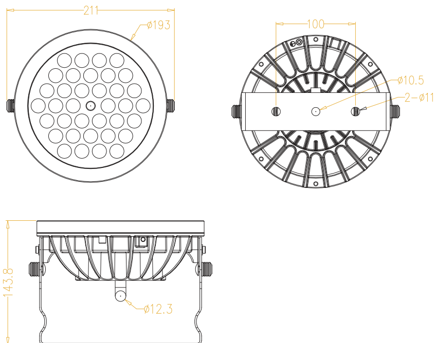
AXS 36 FIXTURE DIMENSIONS – IN-GROUND VERSION
