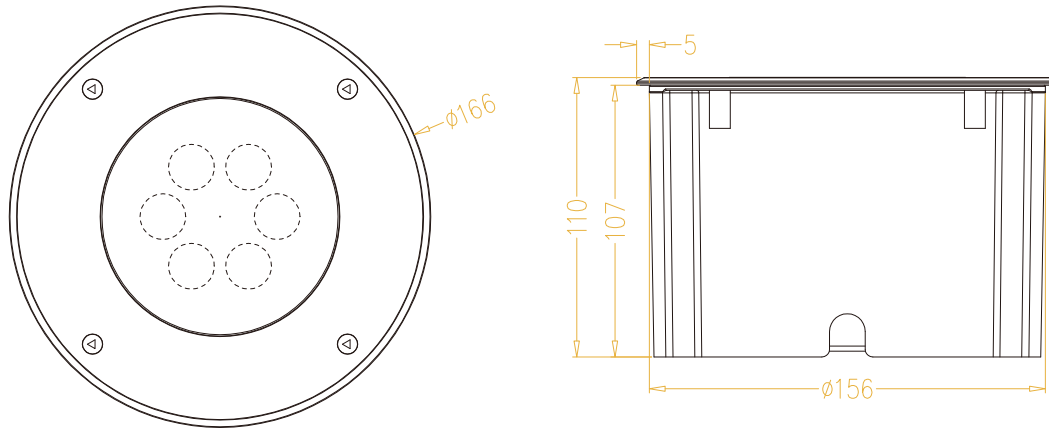
AXS 6 FIXTURE DIMENSIONS
