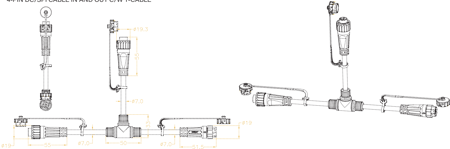
4-PIN DC/SPI CABLE IN AND OUT C/W T-CABLE
