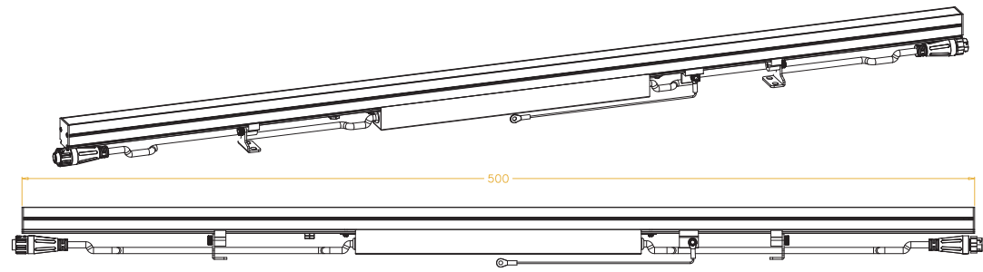
500MM DIMENSIONS WITH ADJUSTABLE BRACKET
