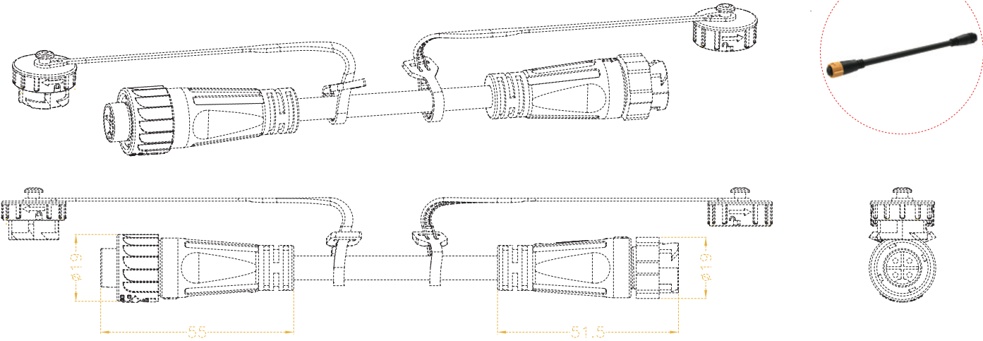
4-PIN DC/SPI CABLE IN AND OUT C/W T-CABLE
