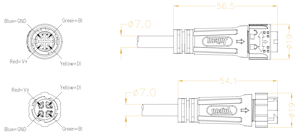
4-PIN DC/SPI CABLE IN AND OUT C/W IP CONNECTOR
