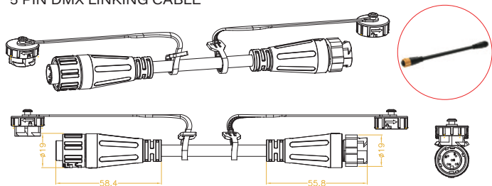
5 PIN DMX LINKING CABLE
