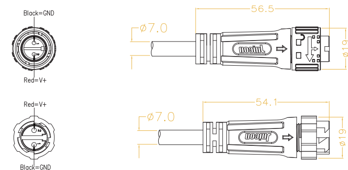
2 PIN SINGLE COLOUR IP CONNECTOR
