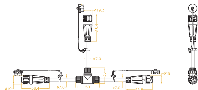
5 PIN DMX IP CONNECTOR
