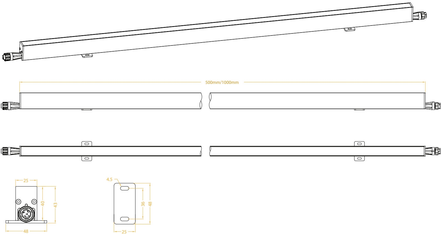
BXG24 DIMENSIONS – FOOT MOUNT
