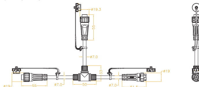
3 PIN SPI T-CABLE
