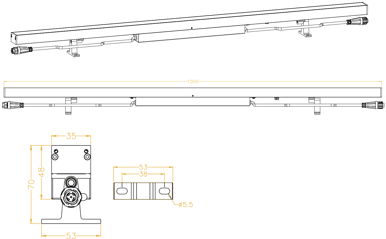
BXG40 DIMENSIONS – 1000MM
