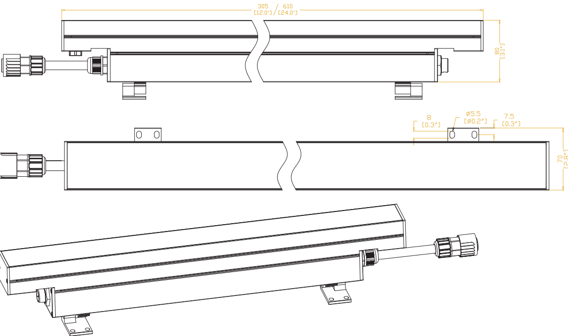
BXG66 DIMENSIONS – 610MM
