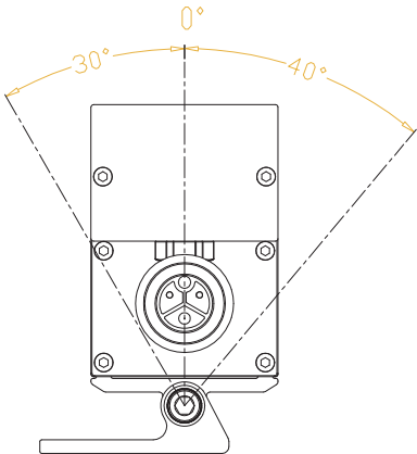
SWIVEL MOUNT
