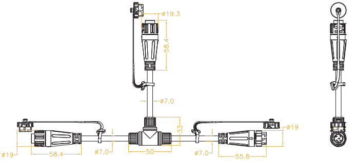
5 PIN DMX T-CABLE
