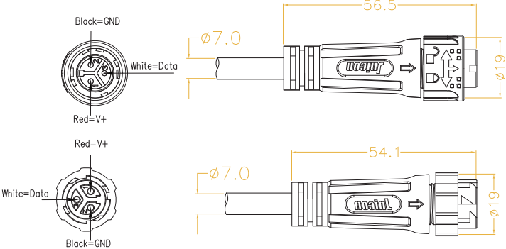
3 PIN SPI IP CONNECTOR
