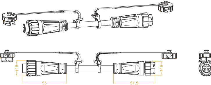
4 PIN X-STREAM LINKING CABLE
