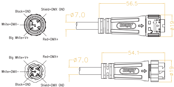
5 PIN DMX IP CONNECTOR
