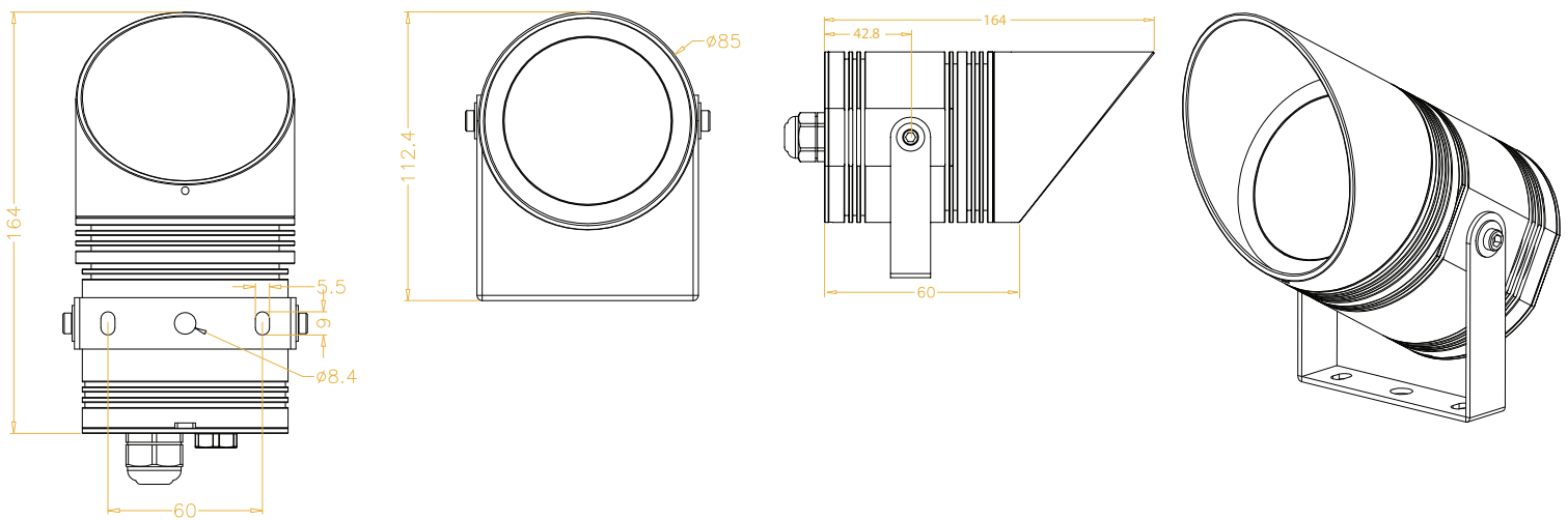
BXS10 DIMENSIONS – HALF SNOOT
