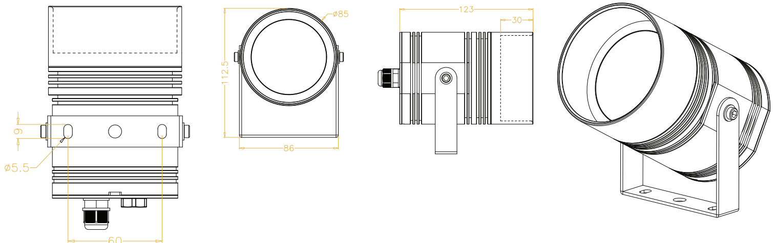
BXS10 DIMENSIONS – FULL SNOOT
