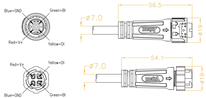
4 PIN X-STREAM IP CONNECTOR
