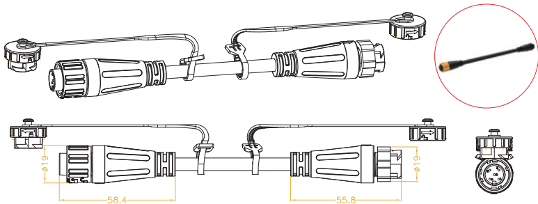
5 PIN DMX LINKING CABLE
