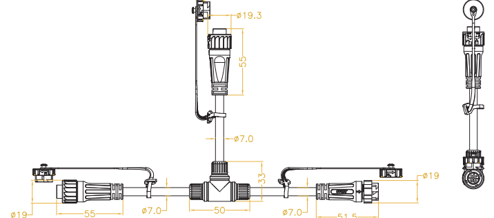
4 PIN X-STREAM T-CABLE
