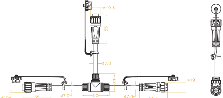
2 PIN SINGLE COLOUR T-CABLE
