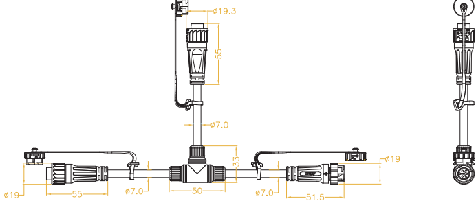
3 PIN SPI T-CABLE
