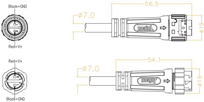
2 PIN SINGLE COLOUR IP CONNECTOR
