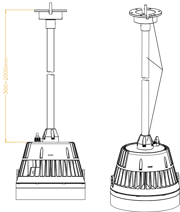
BXS30 – SUSPENSION ROD SYSTEM
