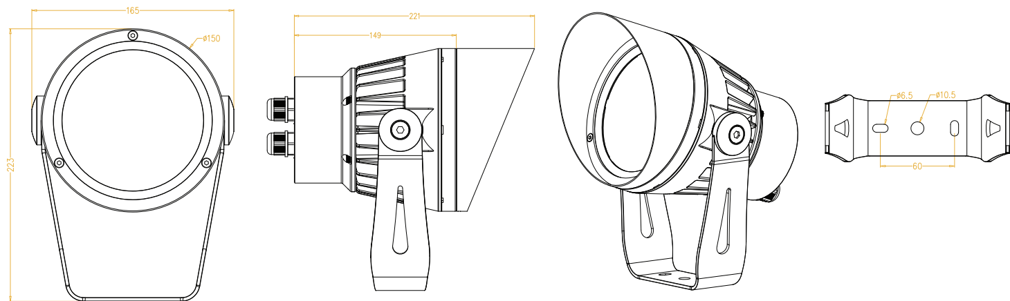
BXS30 DIMENSIONS – HALF SNOOT (WITH BRACKET)
