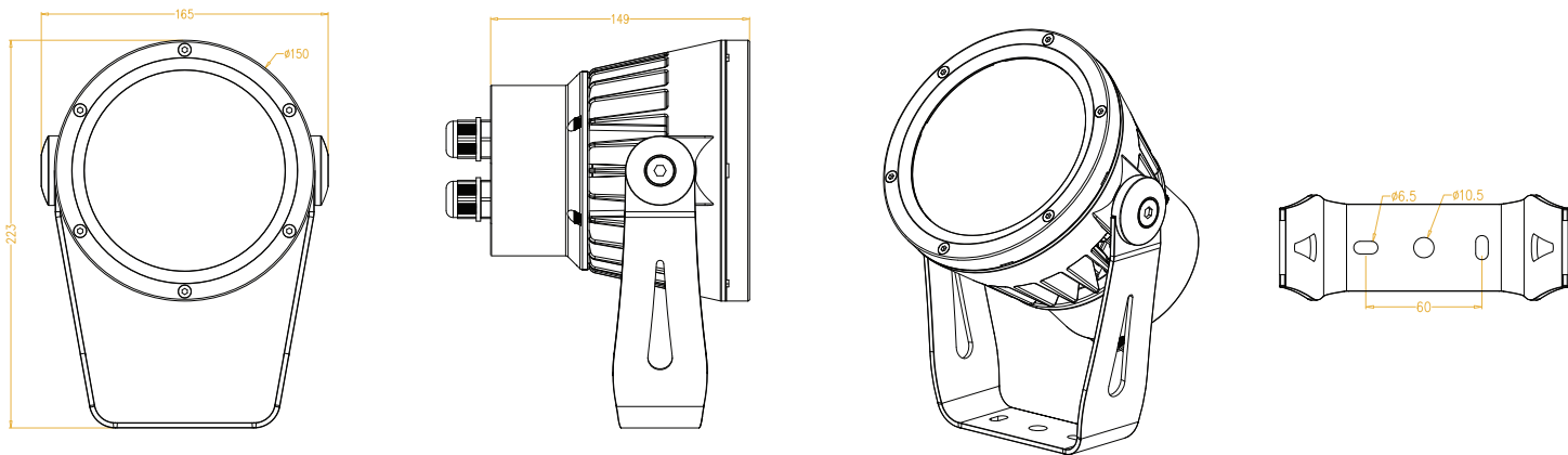
BXS30 DIMENSIONS – NO SNOOT (WITH BRACKET)
