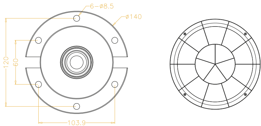
BXS30 DIMENSIONS – CROSSED LOUVER
