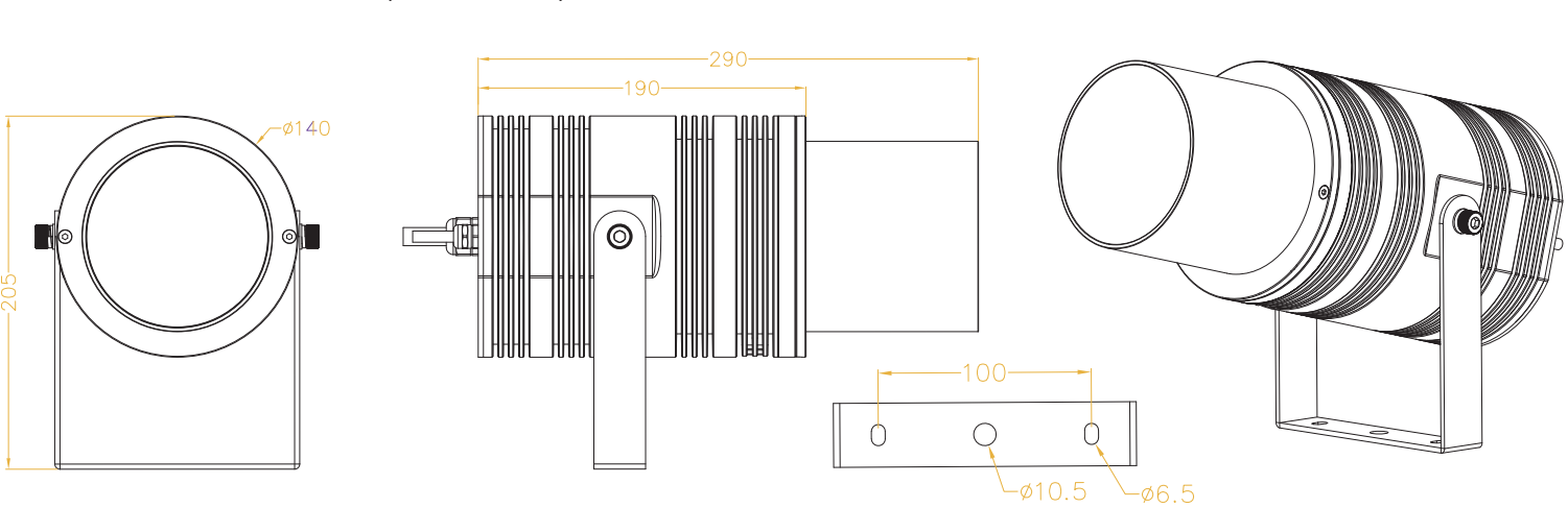
BXS50 DIMENSIONS – FULL SNOOT (WITH BRACKET)
