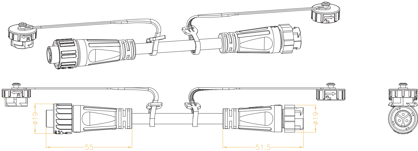
3 PIN SPI T-CABLE
