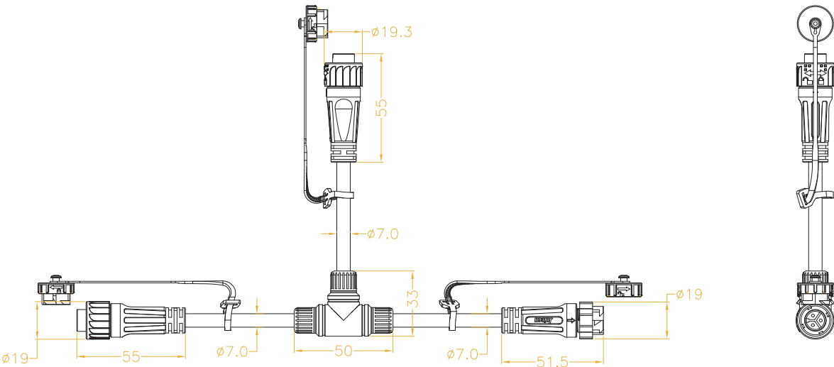
3 PIN SPI T-CABLE
