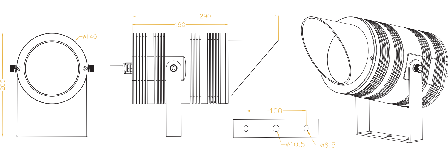
BXS50 DIMENSIONS – HALF SNOOT (WITH BRACKET)
