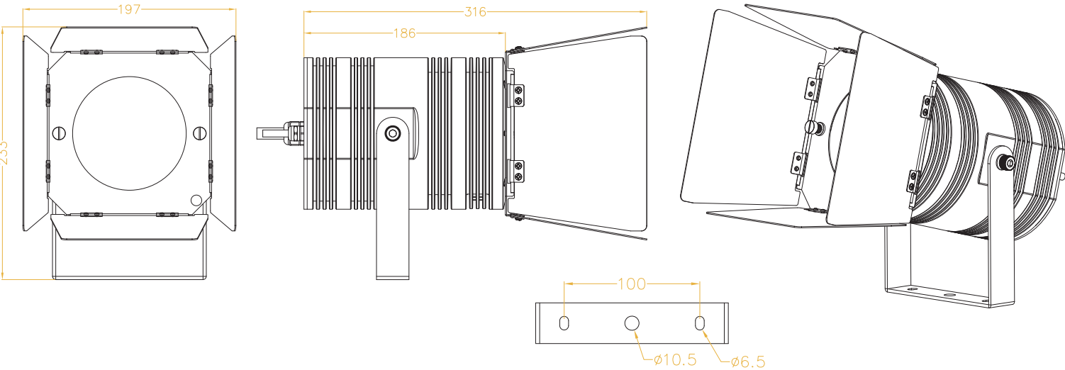
BXS50 DIMENSIONS – BARNDOOR
