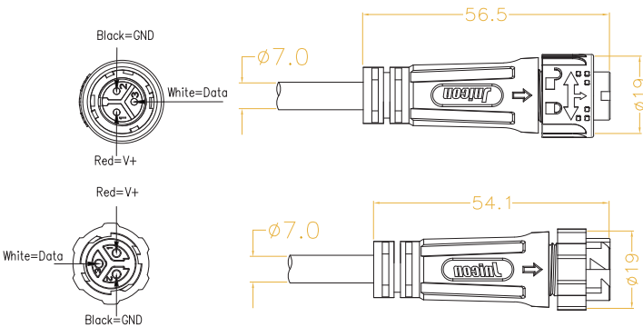
3 PIN SPI IP CONNECTOR
