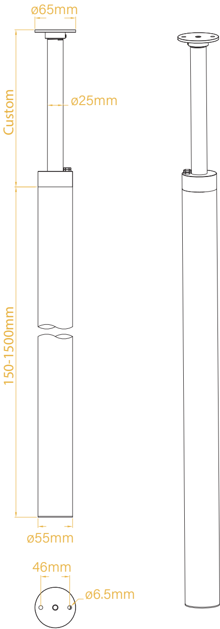
PDX ROD MOUNT DIMENSIONS
