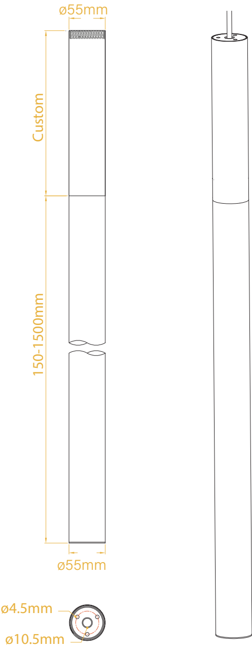
PDX TUBE MOUNT DIMENSIONS
