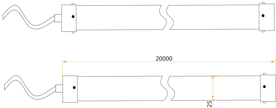
RXN25 DIMENSIONS
