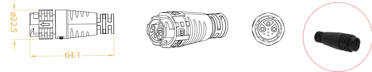
8-PIN AC/SPI + BOOSTER + SENSOR END CAP/IP BLOCK
