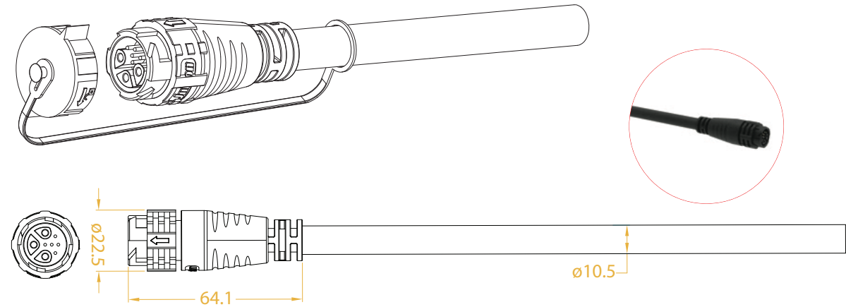
8-PIN AC/SPI + BOOSTER + SENSOR FEED CABLE
