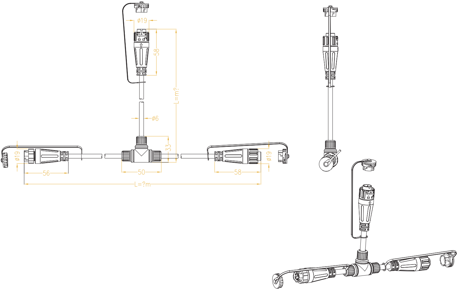
5-PIN DC/DMX T-CABLE
