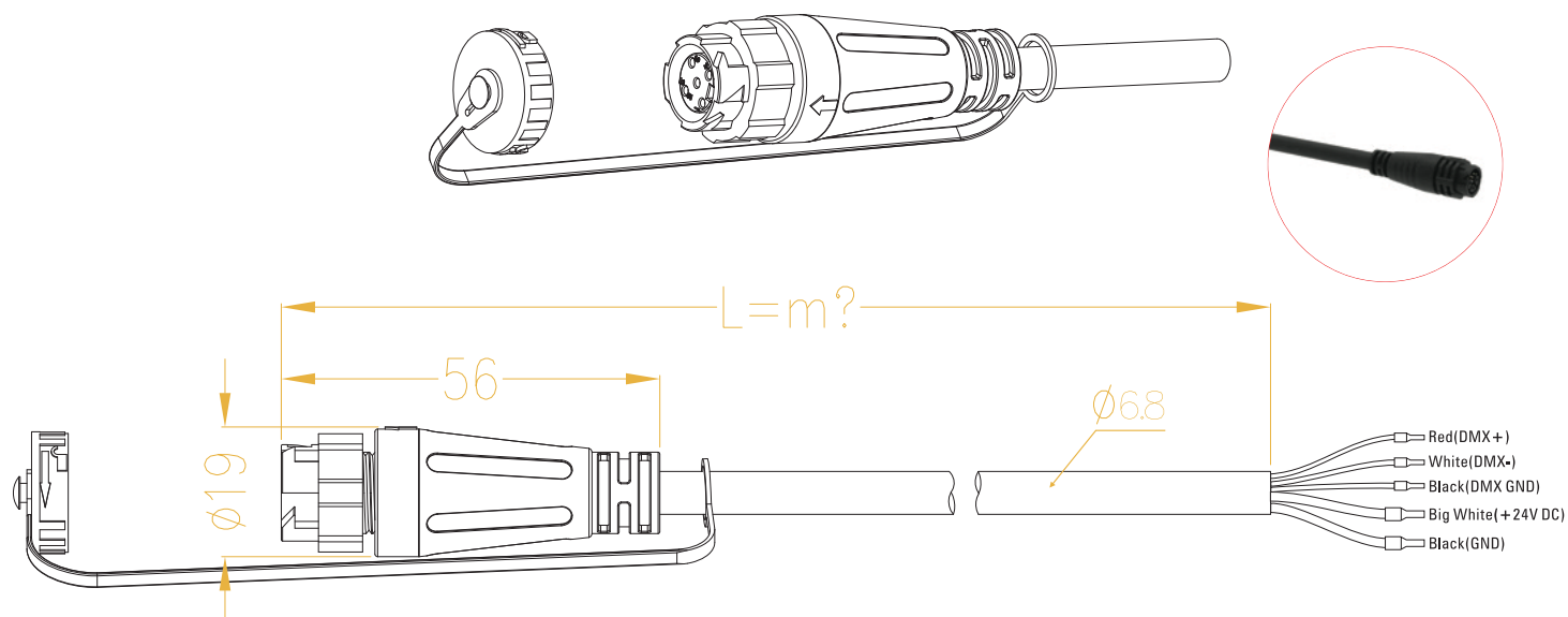
5-PIN DC/DMX LEADER STARTER CABLES
